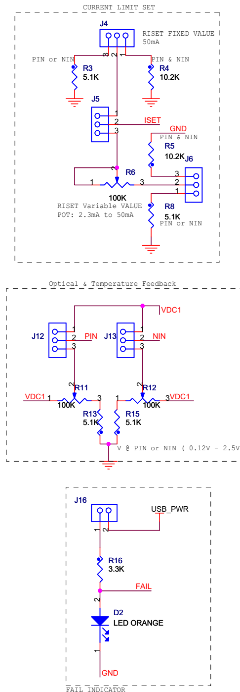
Figure 10. EVB Schematic (3)
